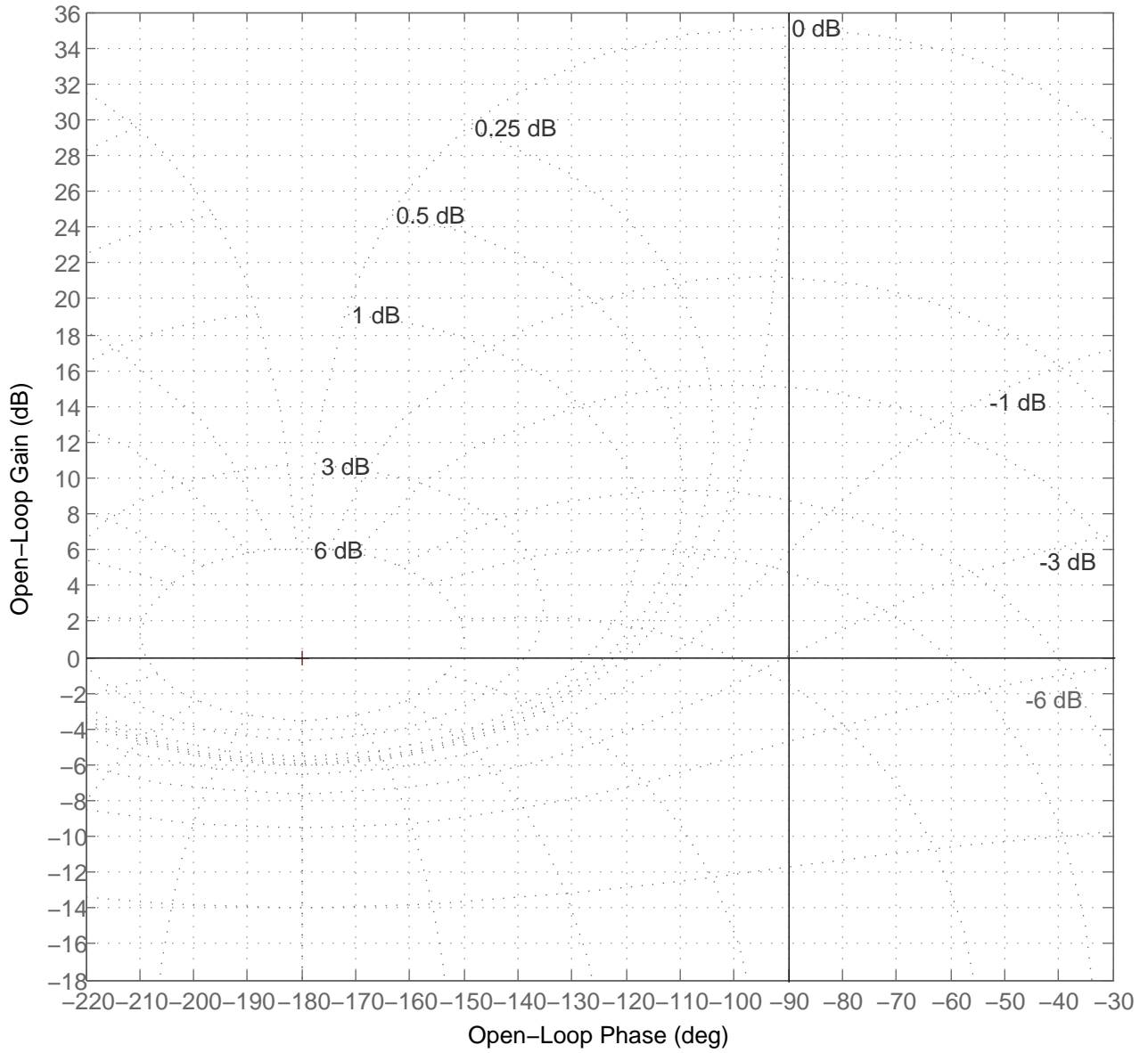
Nichols Chart
